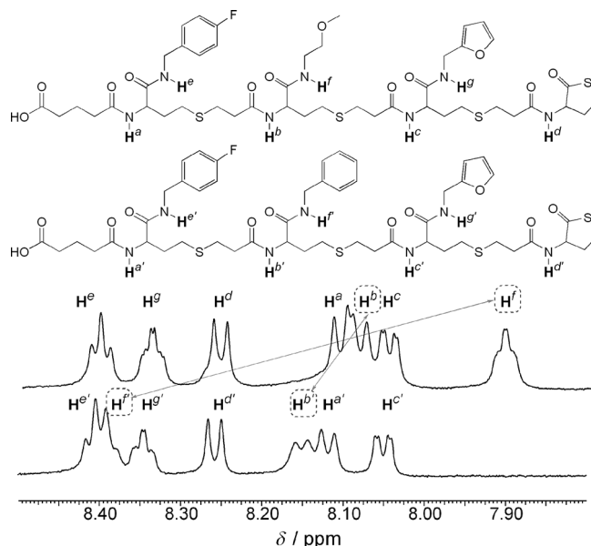
Figure 3. The amide signals in the 1 H NMR spectra (500 MHz, [D 6 ]DMSO) of two structurally related trimeric species.
